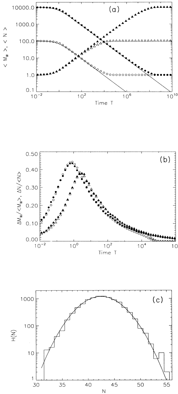
FIG. 1. Nonshattering model: (a) Weight-average mass \langle M_W \rangle (circles) and total number of particles \langle N \rangle (triangles) over time T with a single initial cluster of size L = 10^2 (unfilled symbols) and L = 10^4 (filled symbols). The lines are the corresponding predictions of S(t) from the scaling theory of the continuous fragmentation equation (2) with \omega = 6 \times 10^{-3} and \omega = 7 \times 10^{-9} . (b) Relative rms fluctuations of \Delta N / \langle N \rangle (triangles) and \Delta M_W / \langle M_W \rangle (circles) over time T with a single initial cluster of size L = 10^2 (unfilled symbols) and L = 10^4 (filled symbols). (c) Histogram plot for the total number of particles measured at time T = 10^3 when the initial cluster has size L = 10^2 . The frequency distribution H(N) , obtained from 10^4 realizations, can be fitted by a Gaussian distribution with parameters \bar{x} = 42.5 , \sigma = 3.3 and prefactor A = 996 as shown by the line.
