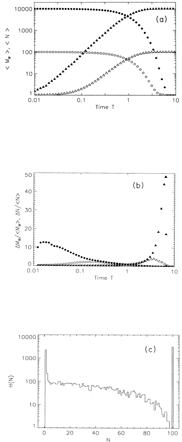
FIG. 2. Shattering model: (a) Weight-average mass \langle M_W \rangle (circles) and total number of particles \langle N \rangle (triangles) over time T with a single initial cluster of size L = 10^2 (unfilled symbols) and L = 10^4 (filled symbols). (b) Relative rms fluctuations of \Delta N / \langle N \rangle (triangles) and \Delta M_W / \langle M_W \rangle (circles) over time T with a single initial cluster of size L = 10^2 (unfilled symbols) and L = 10^4 (filled symbols). (c) Histogram plot for the total number of particles measured at time T = 1.5 when the initial cluster has size L = 10^2 . Here, H(N) is the frequency distribution obtained from 10^4 realizations of the process.
